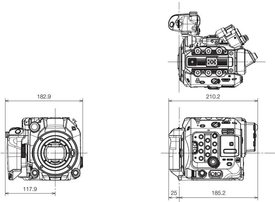
Camera with camera grip and optional EU-V1 Expansion Unit 1
