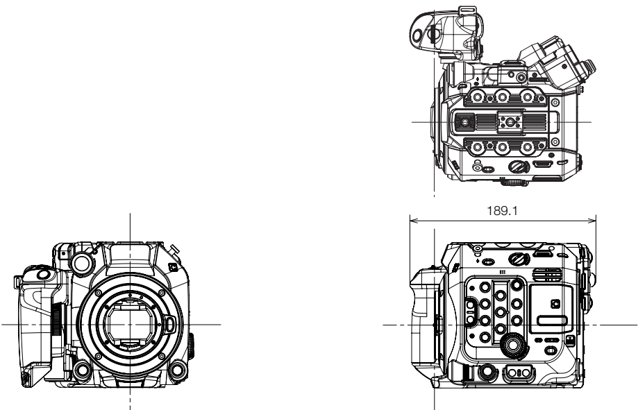
Camera with camera grip
