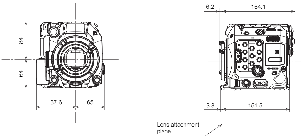
Camera with EF Cinema Lock lens mount
