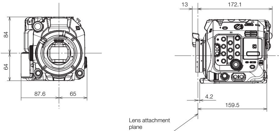
Camera with PL lens mount
