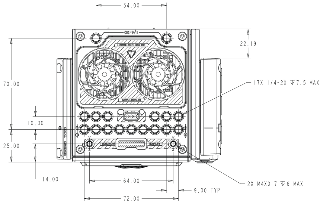
Figure: WEAPON 8K S35 Top View
